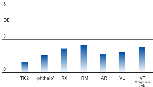
Fig. 1: Pale Shade - standard resin system. Colour difference results after 1000 hours exposure
