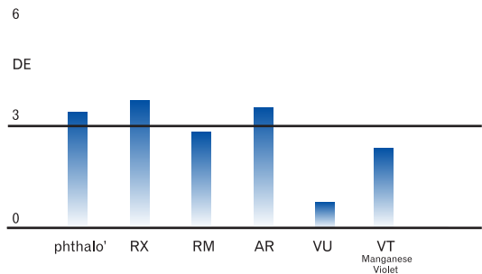
Fig. 2: Deep Shade - standard resin system Colour difference after 1000 hours exposure
