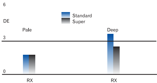
Fig. 3: Performance of Premier RX in standard and super durable systems Colour difference after 1000 hours exposure
